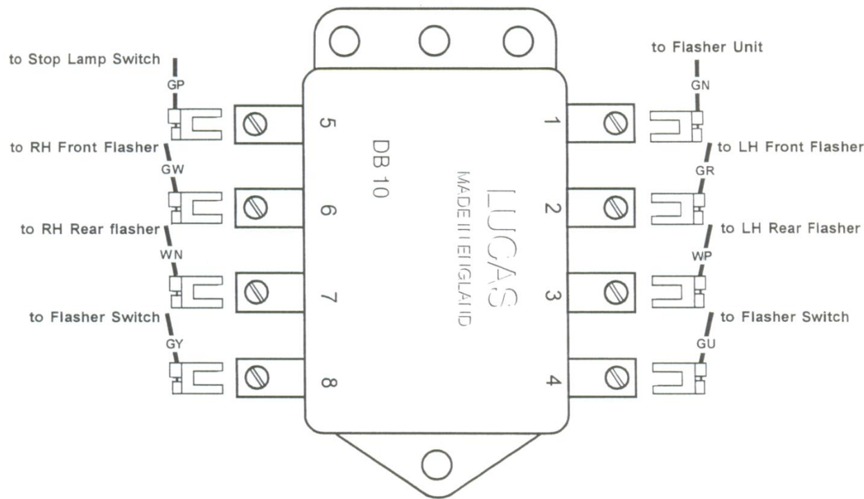
STOP/FLASHER RELAY
